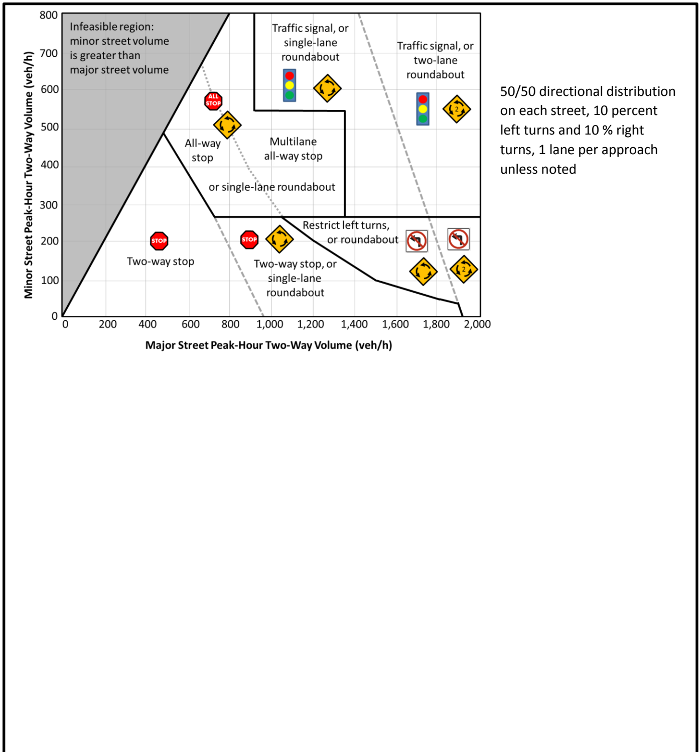
Figure A1: Intersection Control Type by Peak Hour Volume Thresholds 6
